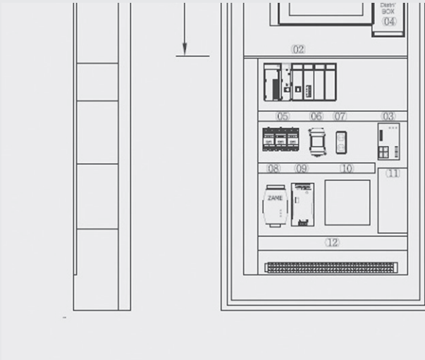
(1) (모델명: VPM-MP-01)
